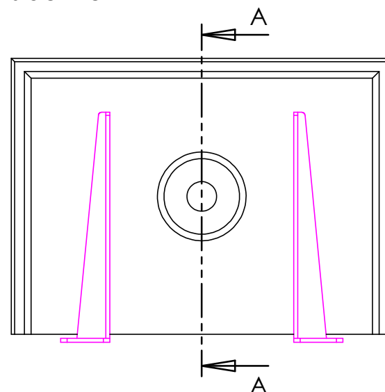
Underside View
